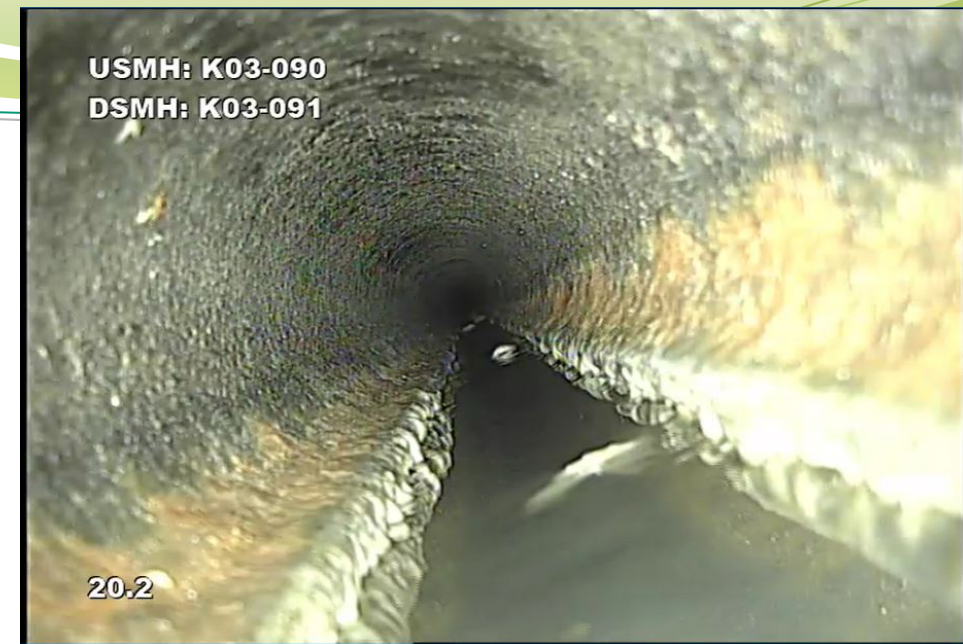
Grease accumulation downstream of Lucille's – CCTV on February 13, 2023
